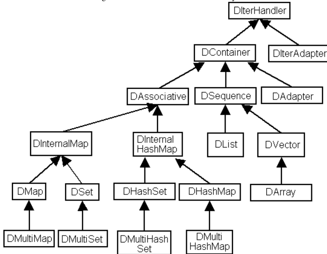
Figure 11.1: SDL container class hierarchy:
